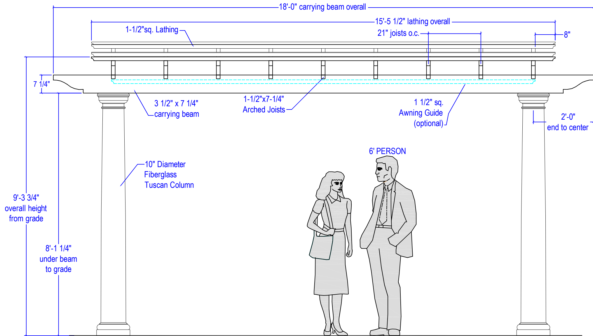
1 10x14 & 12x14 Side View (Arched) not to scale
