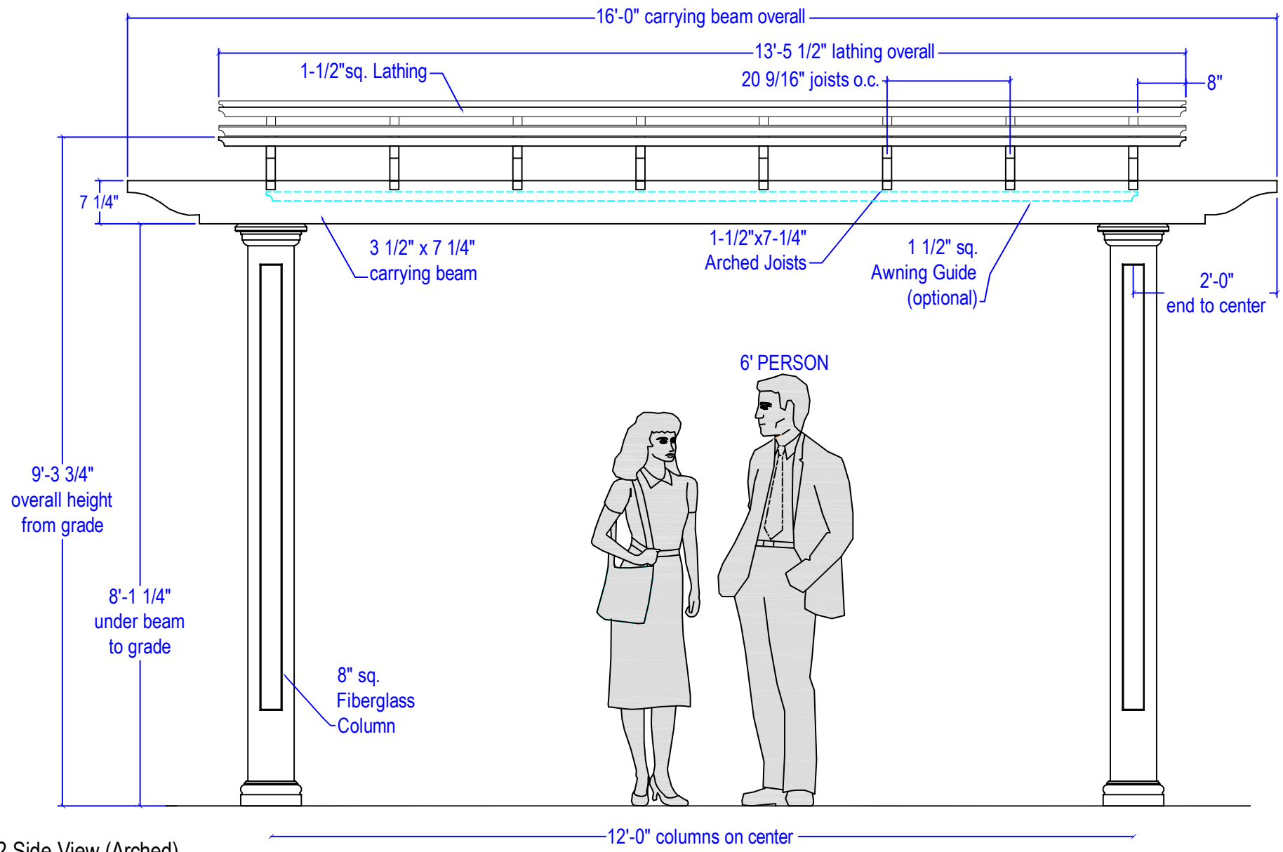
1 10x12 & 12x12 Side View (Arched) not to scale
