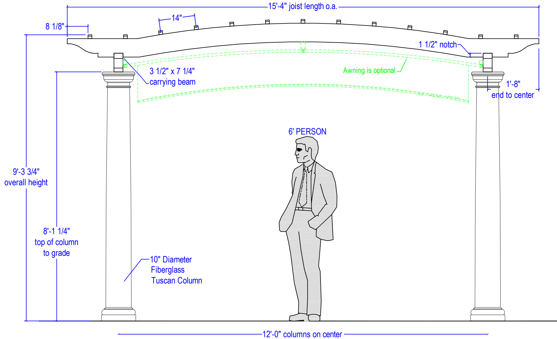
1 12x End View (Arched) not to scale
