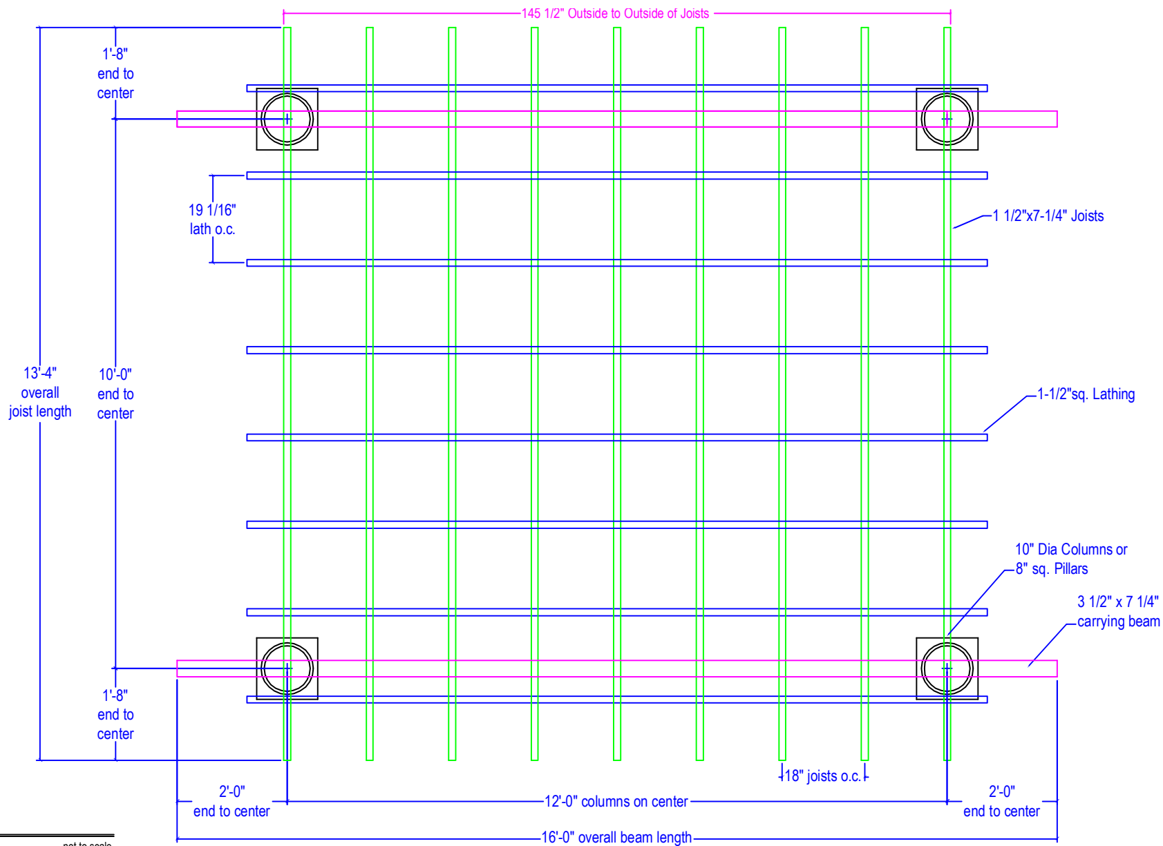
1 10x12 Plan View Flat Top SKU# 795386
