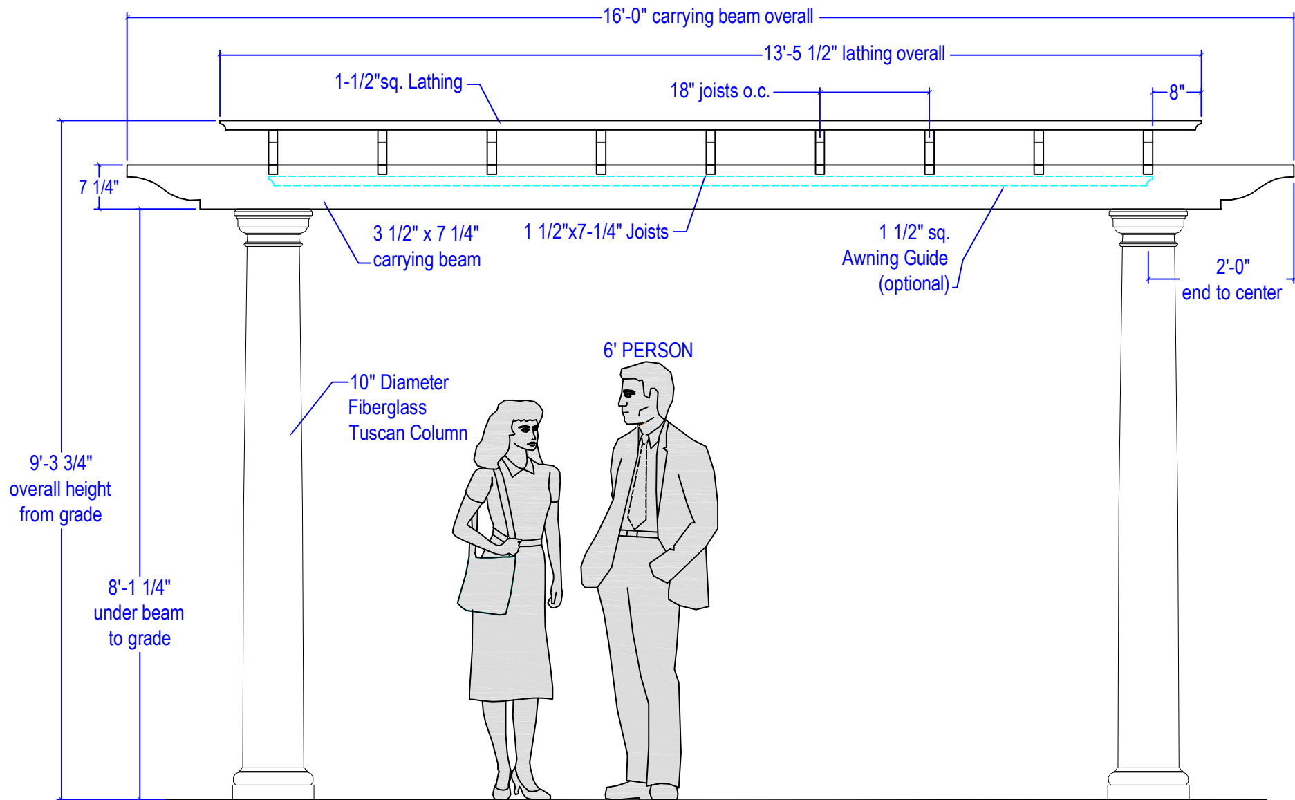
1 10x12 & 12x12 Side View (Flat)
